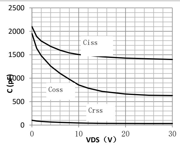
Fig.2 Capacitance Characteristics
